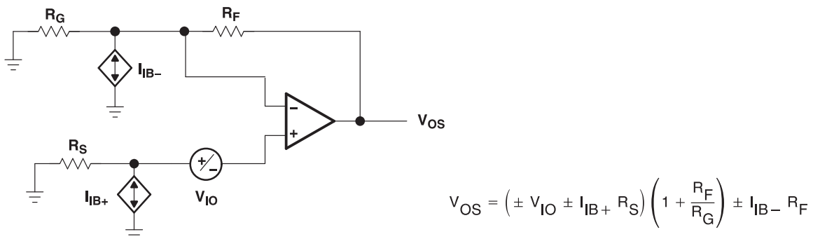
Figure 48. Output Offset Voltage Model
